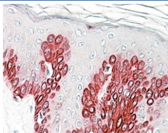
IHC staining of FFPE human skin with Sirtuin 1 antibody at 4ug/ml. HIER: steamed with pH6 citrate buffer, AP-staining.
