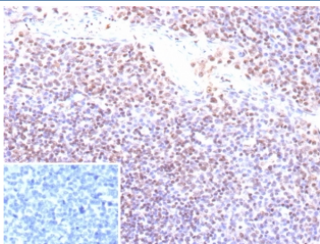
IHC staining of FFPE human tonsil tissue with recombinant EBV antibody (clone EBV/9620R). Inset: PBS used in place of primary Ab (secondary Ab negative control).
