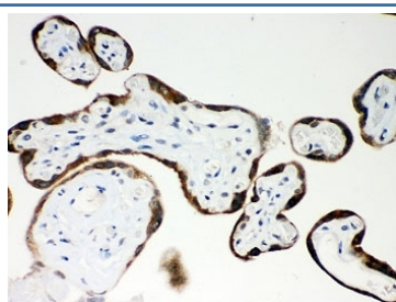
IHC-P: PAPP A antibody testing of human placenta tissue
