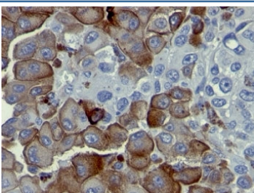
IHC analysis of formalin-fixed, paraffin-embedded human melanoma stained with p75NTR antibody (clone NGFR5).
