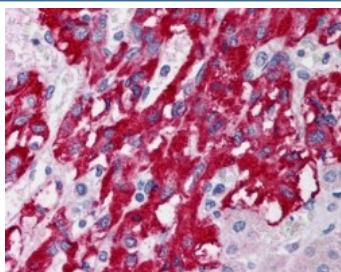
IHC testing of FFPE human adrenal gland with DLC1 antibody at 5ug/ml. HIER: steamed with pH6 citrate buffer, AP-staining.
