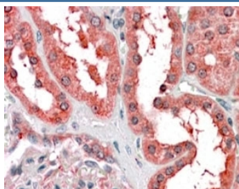
IHC testing of FFPE human kidney with Cyt19 antibody at 4ug/ml. HIER: steamed with pH6 citrate buffer, AP-staining.
