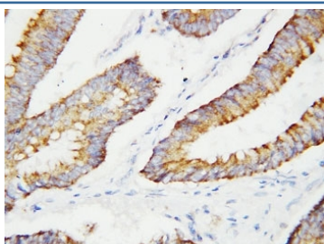
IHC-P: BCAT2 antibody testing of human colon cancer tissue
