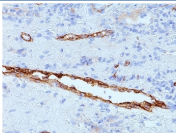
IHC: Formalin-fixed, paraffin-embedded human tonsil stained with anti-vWF antibody (clone IIIE2.34).
